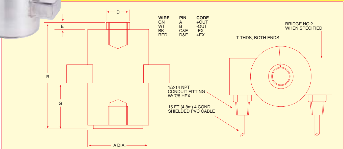
Dimensions Shown in Inches (mm)
